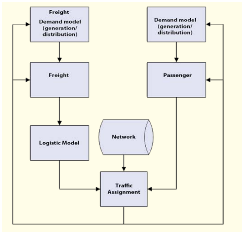
Figure 8: Trans-Tools structure
